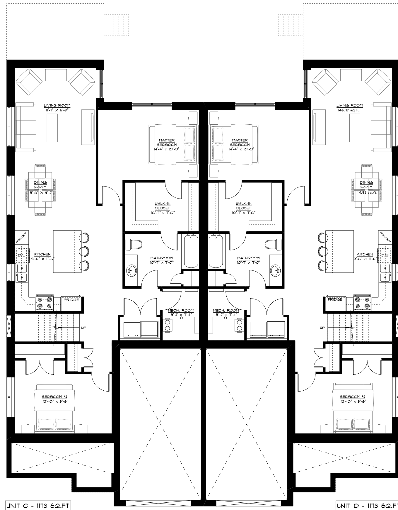
BASEMENT PLAN
